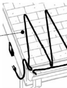
Figure 15. Attaching clips along rise of larger triangles
