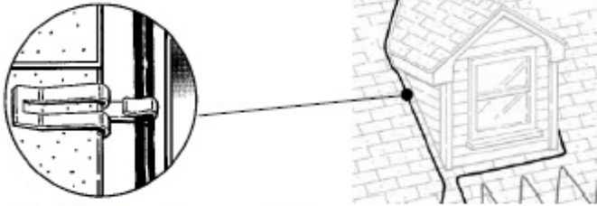
Figure 16. Attaching clips around dormers
